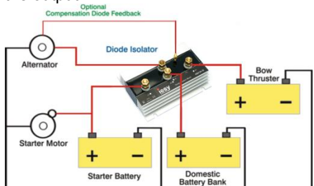
Schematic DB 120-3C
